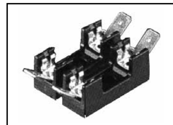
1/4" QUICK CONNECT STYLE
